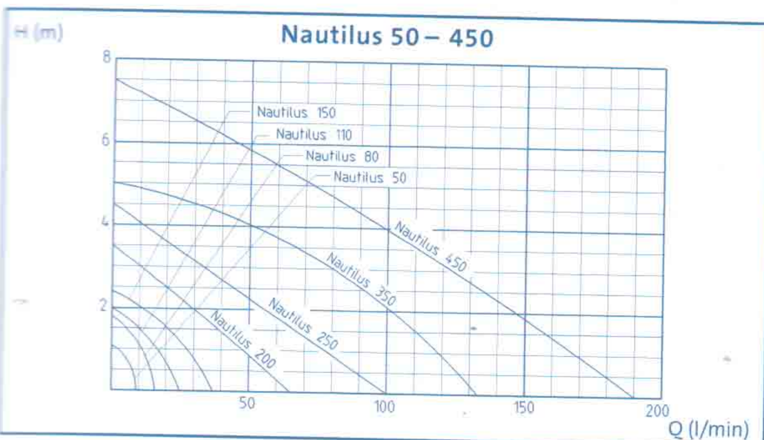
Comparison of pump performance curves, s. p. 132 – 135.
